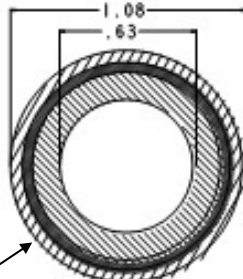
RETURN HOSE (M 25-85) - (1500 PSI)
