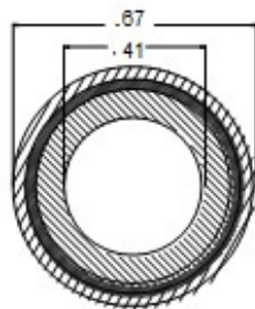
RETURN HOSE (M 3-10) - (2000 PSI)
