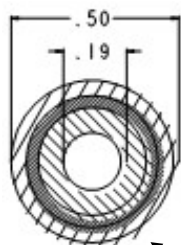
PRESSURE HOSE (3000 PSI)
